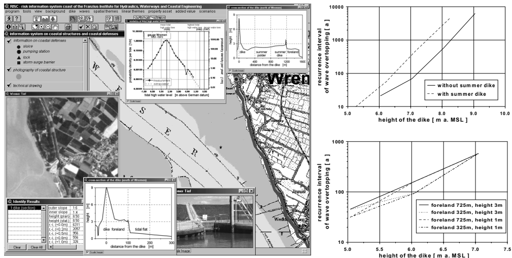
Figure 1 Screenshot of RISC: Locations, profiles and photographs of sea dikes at the estuary Weser (left) and recurrence interval of wave overtopping at sea dikes with or without an additional summer dike (top right) and with different geometries of the foreland (bottom right).
